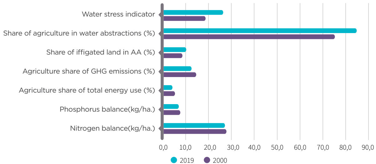
Figure 14. Environmental Indicators in Turkey Source: OECD, 2021c
