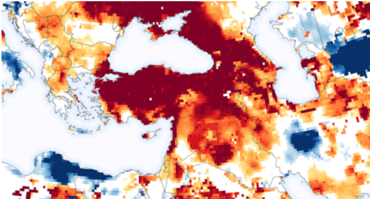
Figure 22. Groundwater Levels of Turkey Source: NASA, 2021
