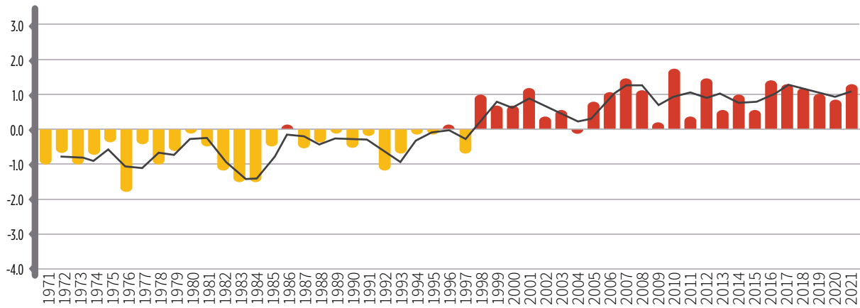
Figure 21. Turkey Average Temperature Anomalies in Summer* 6 Source: MoAF, 2021
