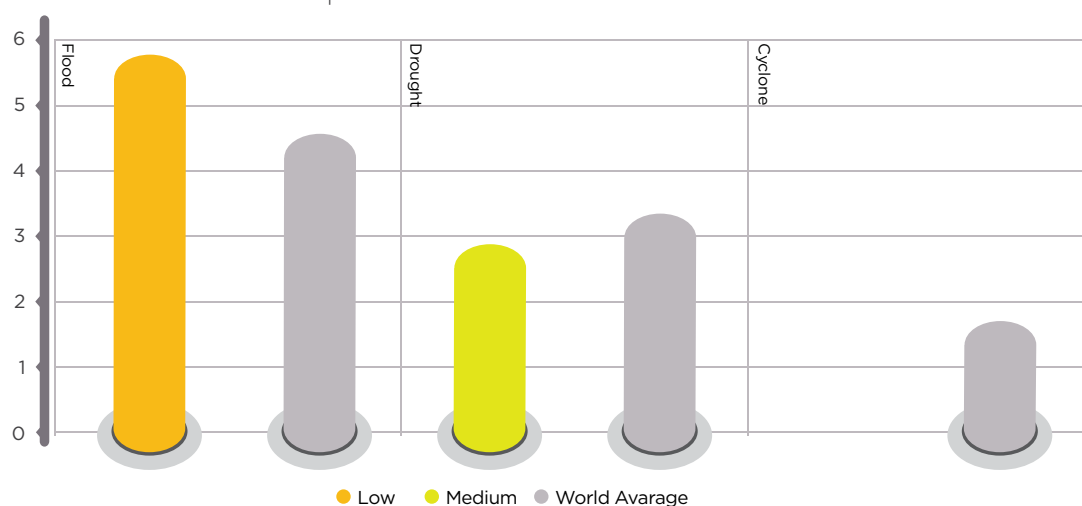
Figure 19. Level of floods, drought and tropical cyclones in Turkey, 2000-2020 Source: IEA, 2020
