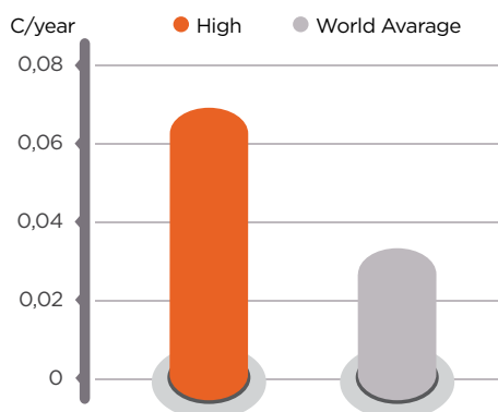
Figure 20. The level of warming in Turkey, 2000-2020 Source: IEA, 2020
