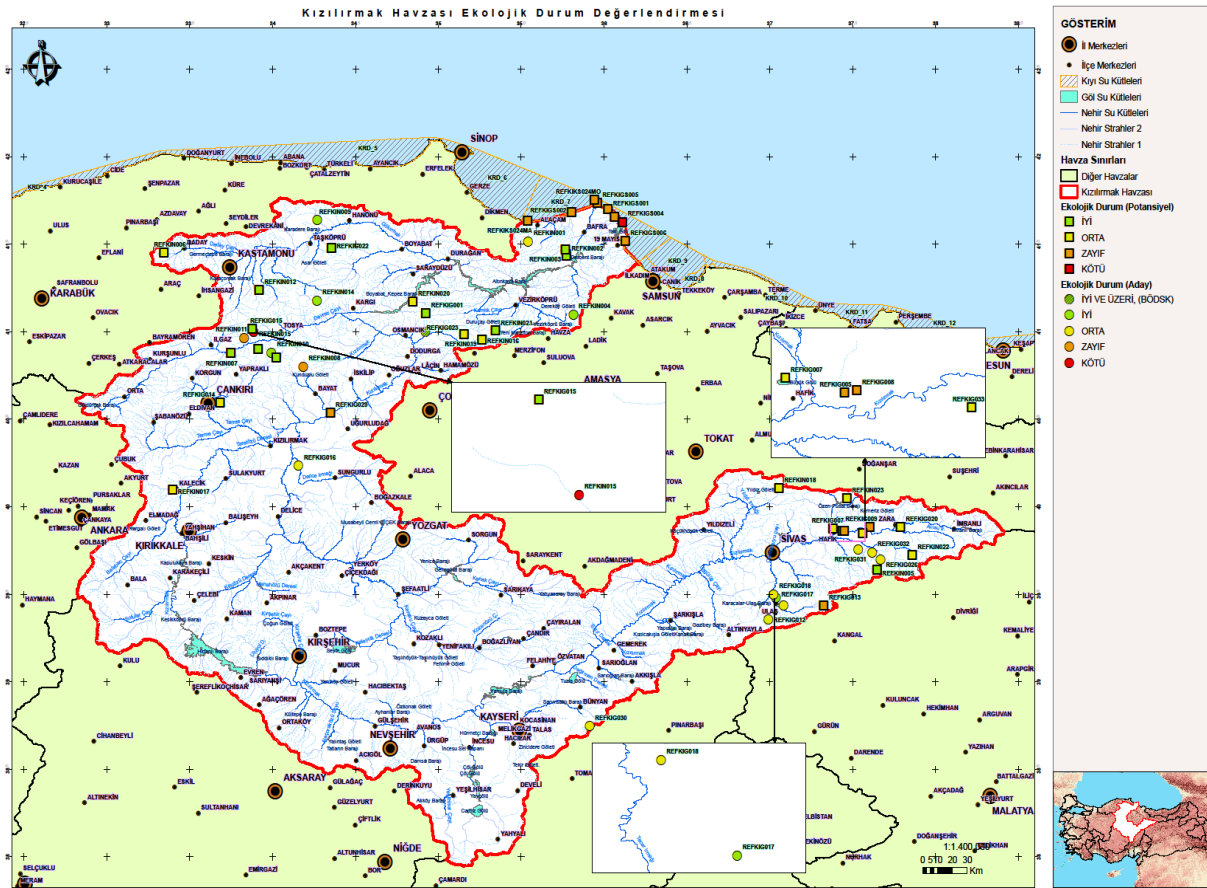
Ecological Status Assessment Results in the Kızılırmak River Basin
